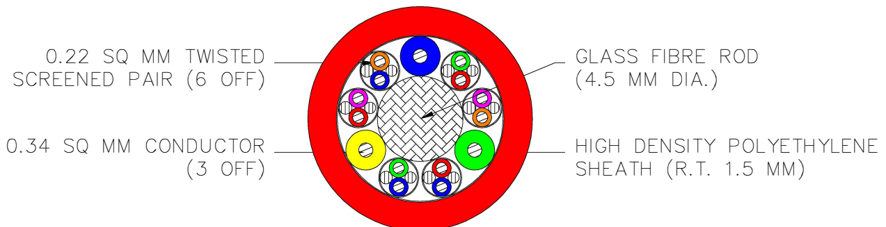
DRAWING No. 1697
