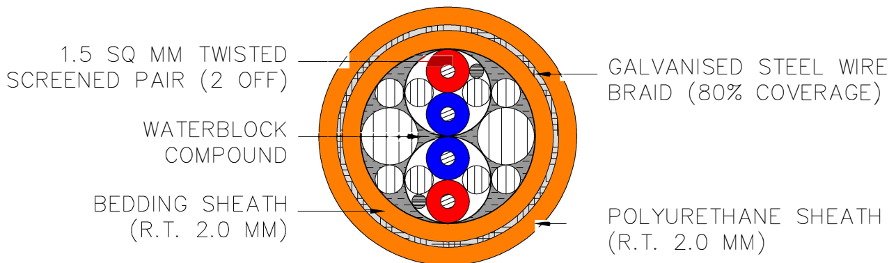
Drawing No. CLS 755
