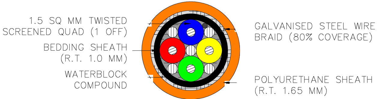
Drawing No. CLS 911
